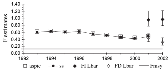
Figure 3. Comparison of estimates of fishing mortality for hogfish based on different assessment methods and data sources: non-equilibrium production model (aspic), stock-synthesis model (ss), and fishery-dependent average length (FD Lbar) methods used Florida-wide data; fishery-independent average length (FI Lbar) method used only Florida Keys RVC data (horizontal line: management benchmark F_{msy} ).
